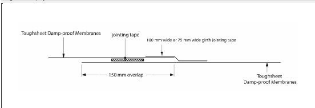
Figure 1 Tape joint
