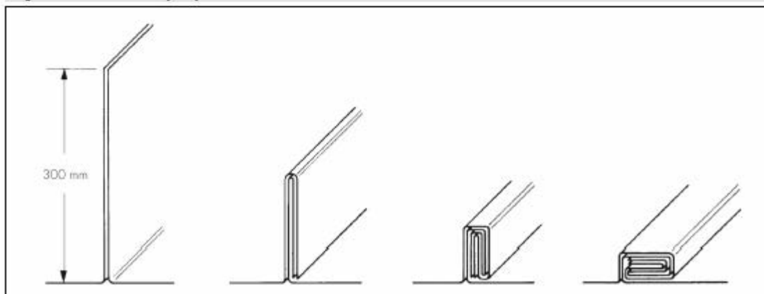
Figure 2 Double-welted fold joint
